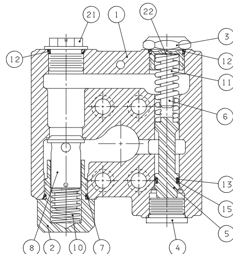
Inlet Relief Valve Before July 2003
