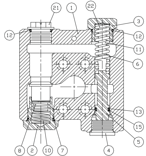
Inlet Check Valve After July 2003
