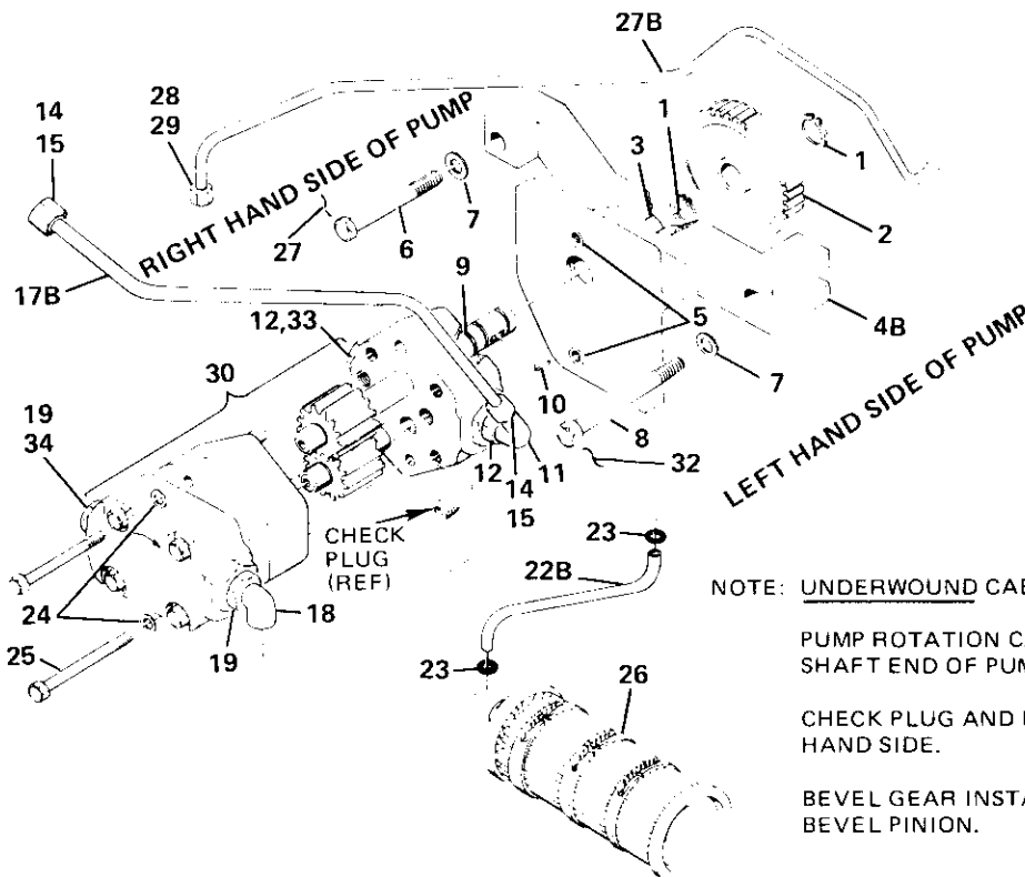
PUMP GROUP 51349-2
