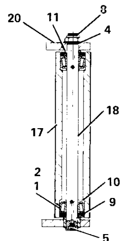
SECTION B-B (VERTICAL ROLLER)
