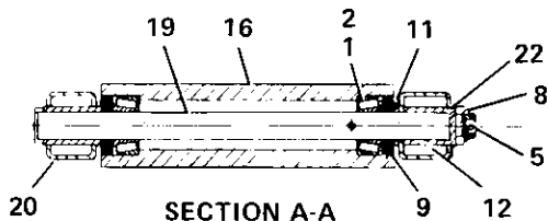
SECTION A-A (HORIZONTAL ROLLER)
