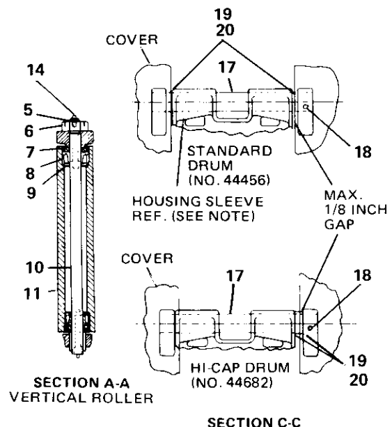
SECTION C-C
