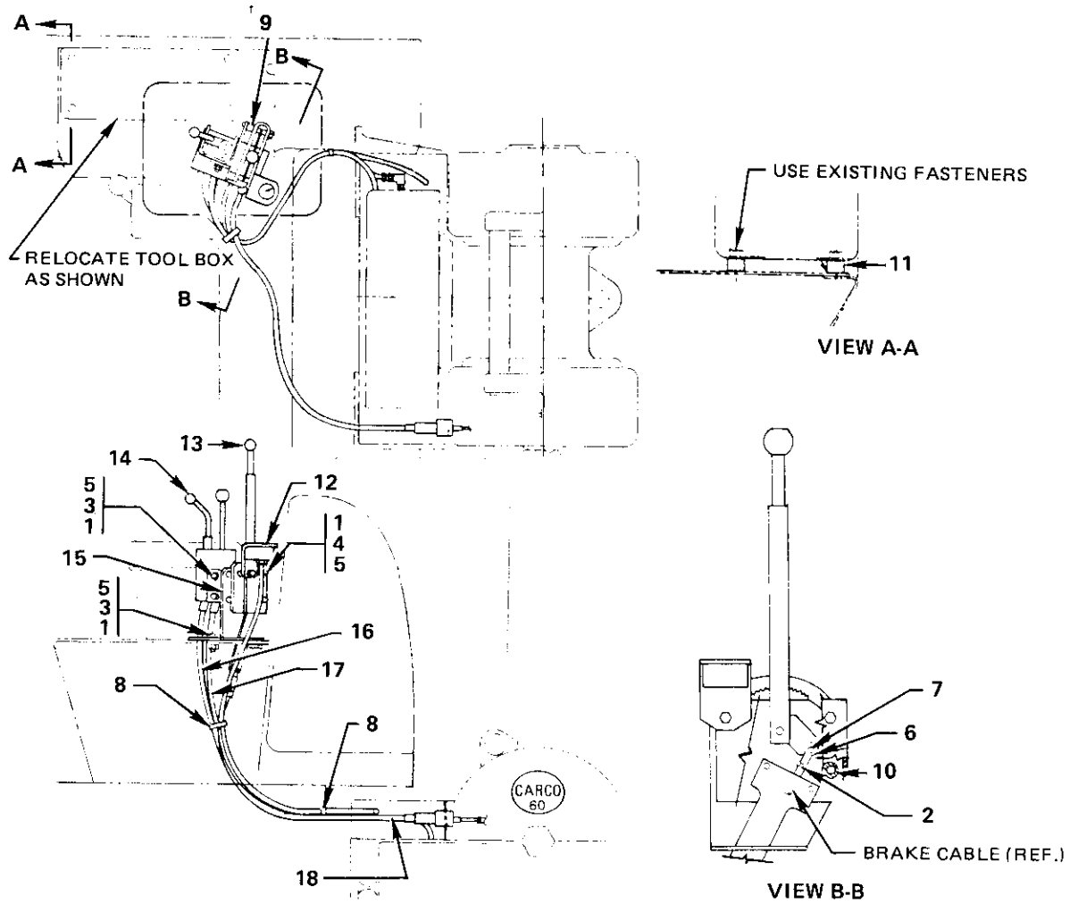
CONTROL GROUP (PSM AND PSC WITH FREE SPOOL) NO. 52263
