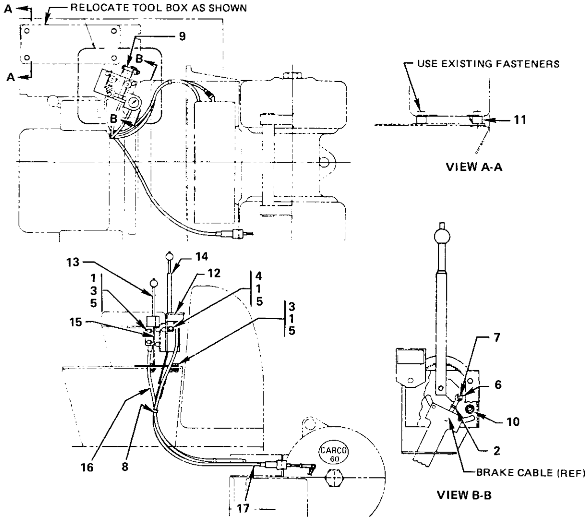
CONTROL GROUP (PSM AND PSC WITHOUT FREE SPOOL) NO. 52262
