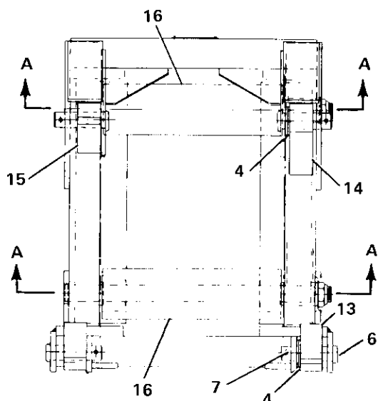
FAIRLEAD ASSEMBLY
