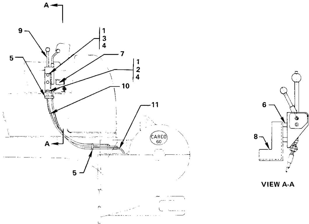
CONTROL GROUP (P.S. WITH FREE SPOOL) NO. 52261
