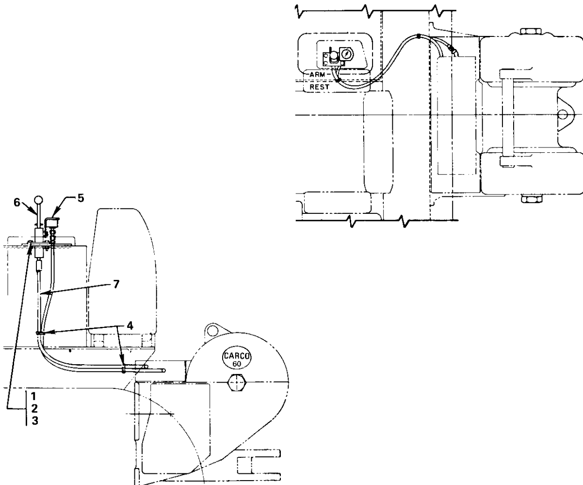
CONTROL GROUP (P.S. WITHOUT FREE SPOOL) NO. 52039
