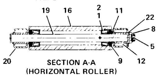
FAIRLEAD ASSEMBLY
