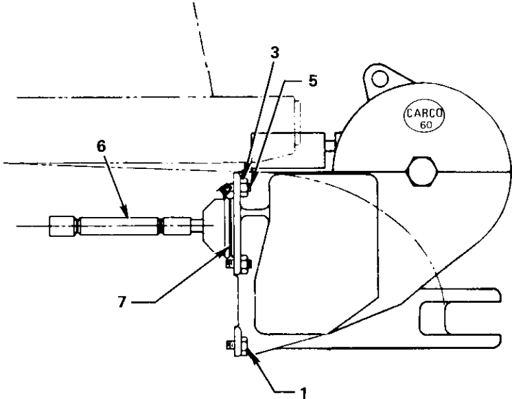
VIEW OF TRACTOR, REAR FACE
