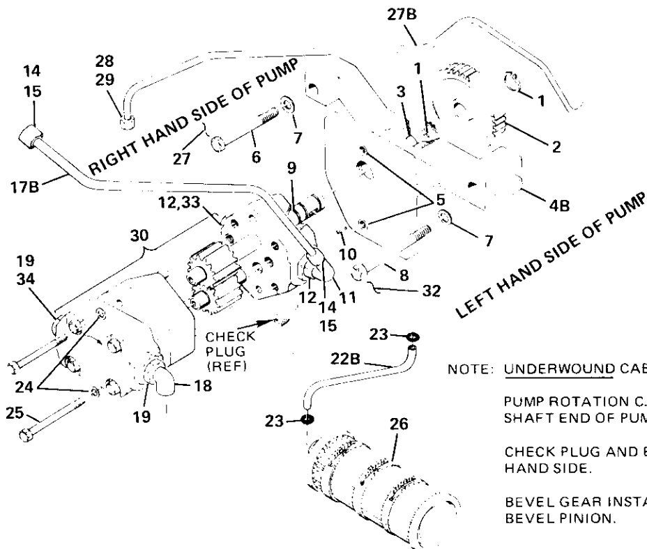
PUMP GROUP 51349-2
