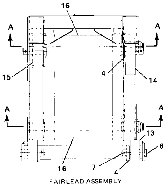
FAIRLEAD ASSEMBLY
