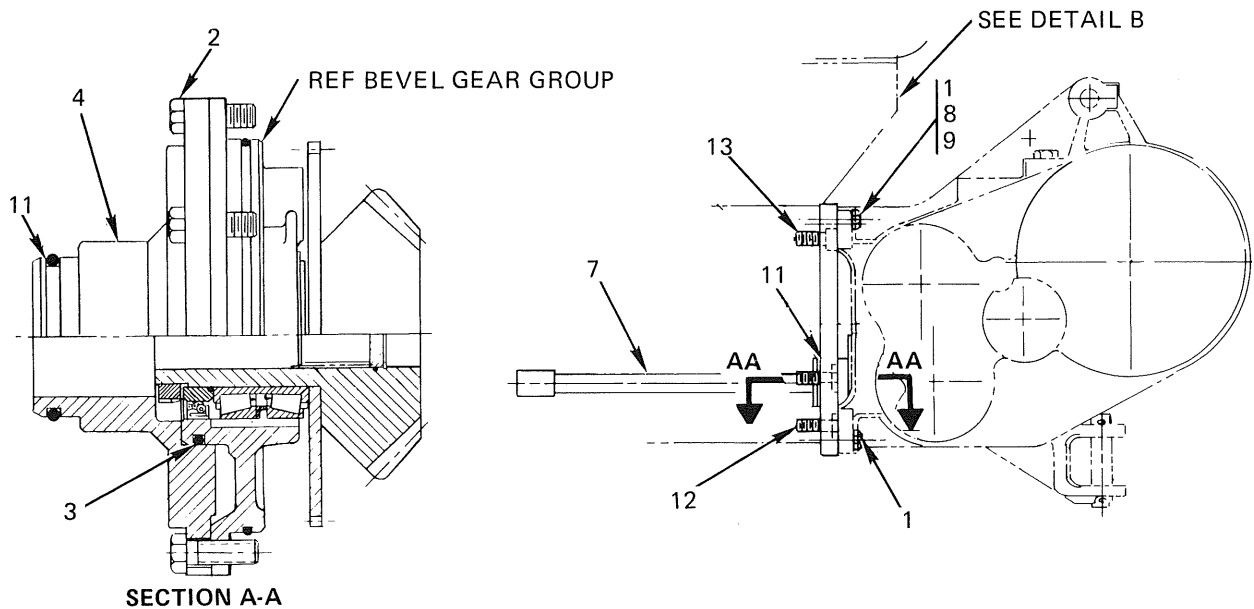
MOUNTING GROUP – 53174-53175 FA 10C
