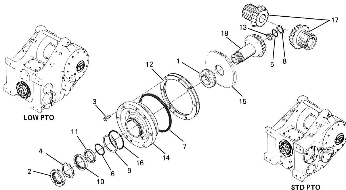
BEVEL GEAR SET 53120-0104 STD OR 53120-0105 SLOW SPEED
