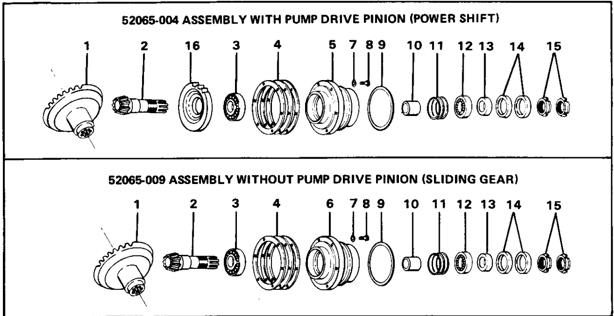
GEAR SET NO. 52065-104 RATIO 1.56/1
