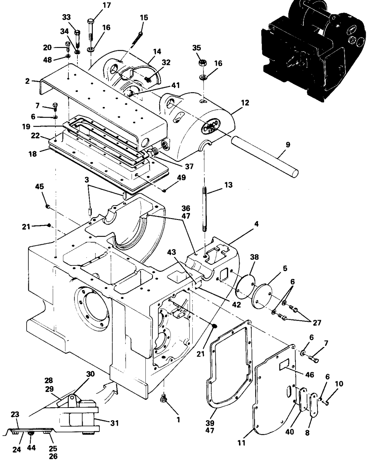
WINCH CASE
