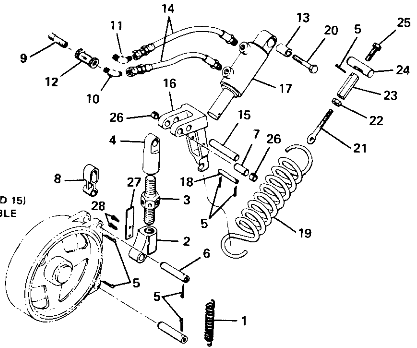
PS BRAKE CONTROL (SPRING APPLIED) GROUP NO. 52076
