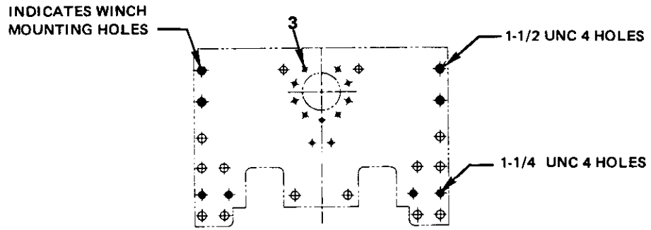
VIEW OF TRACTOR REAR FACE
