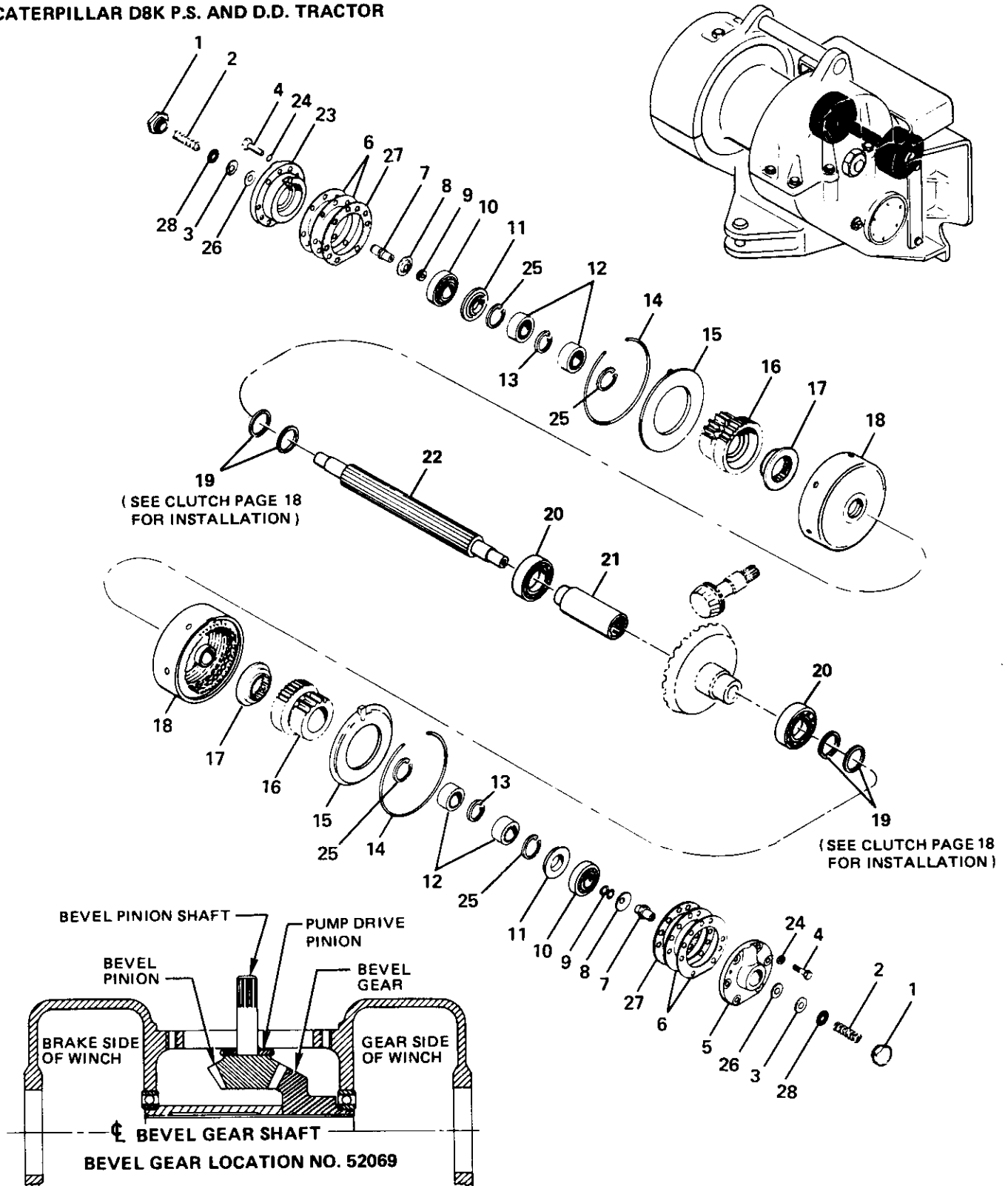
BEVEL GEAR SHAFT GROUP NO. 52273
