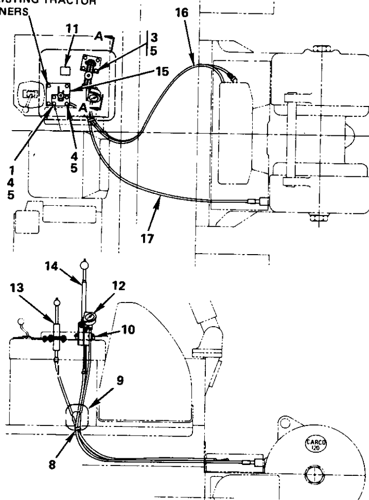
CONTROL GROUP (PSM & PSC WITH MANUAL BRAKE) NO. 51938
