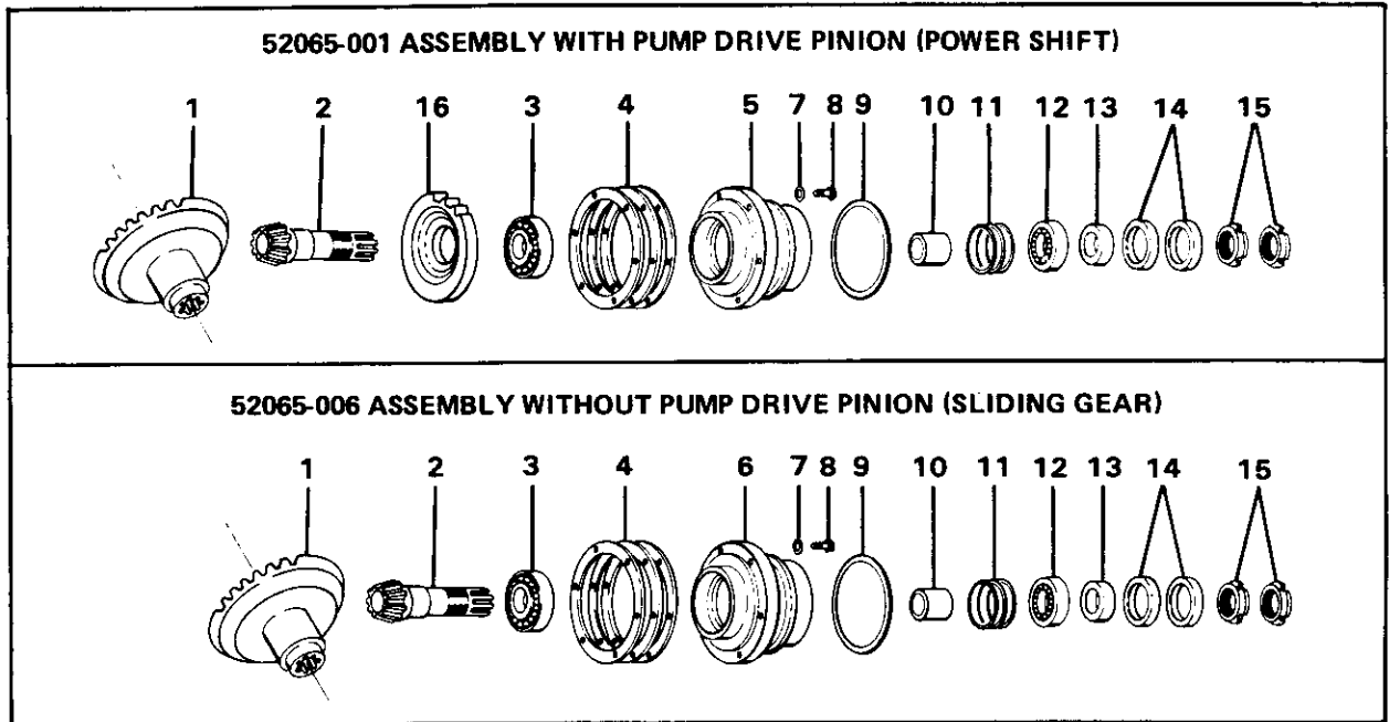
GEAR SET NO. 52065-101 RATIO 2.59/1
