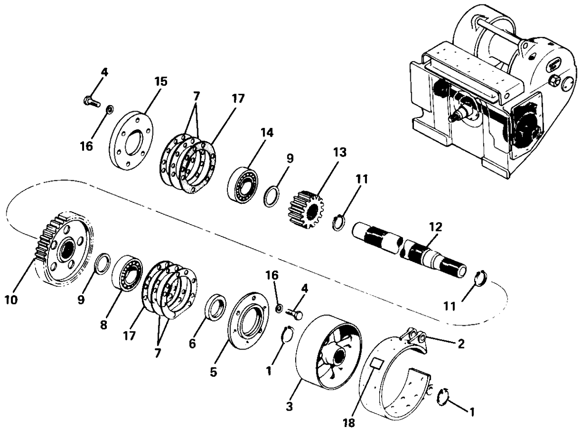
BRAKE SHAFT GROUP NO. 52277
