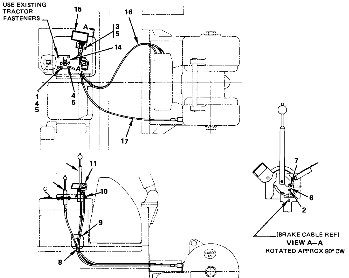
CONTROL GROUP (PS WITH 2 IN 1 INCHING BRAKE ) NO. 51937
