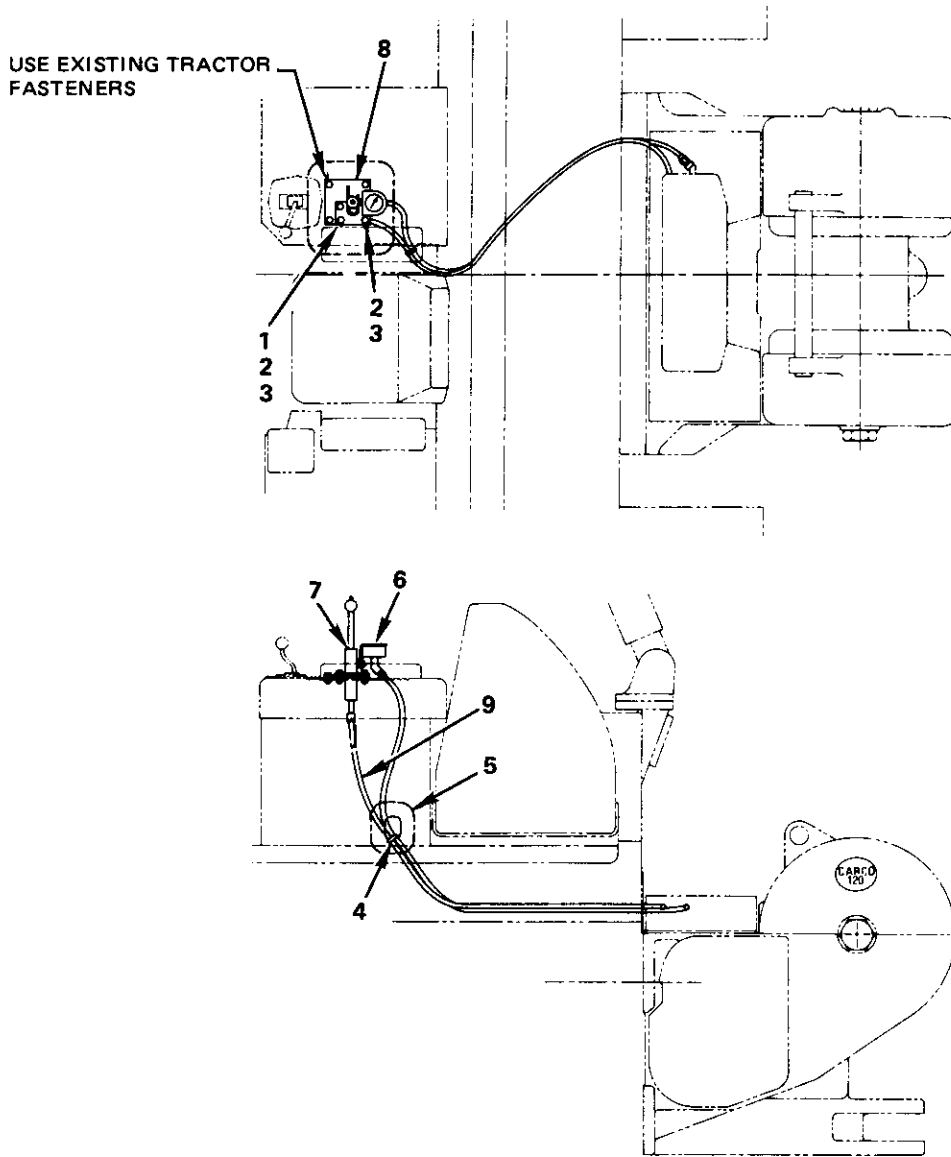
CONTROL GROUP (PS) NO. 51936
