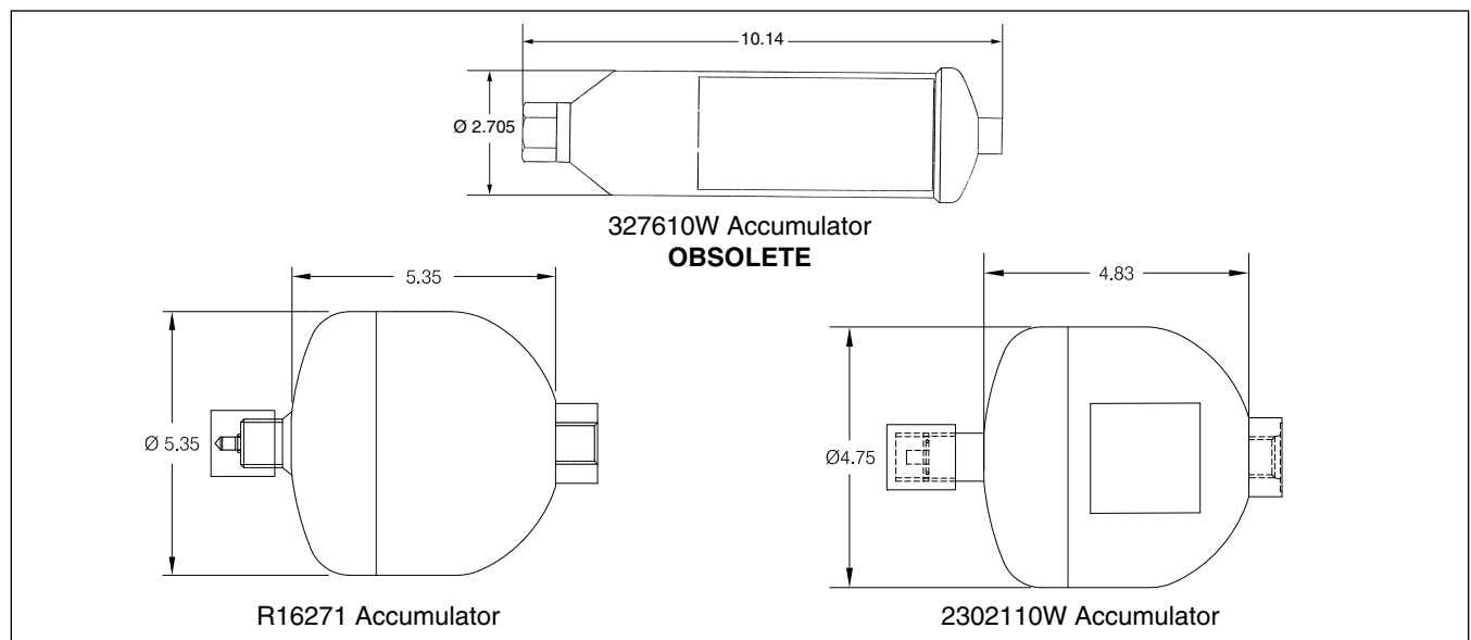
Figure 1: Accumulators
